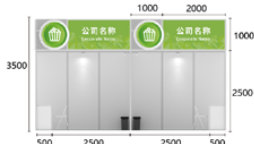
展位侧面图 Side elevation of booth
